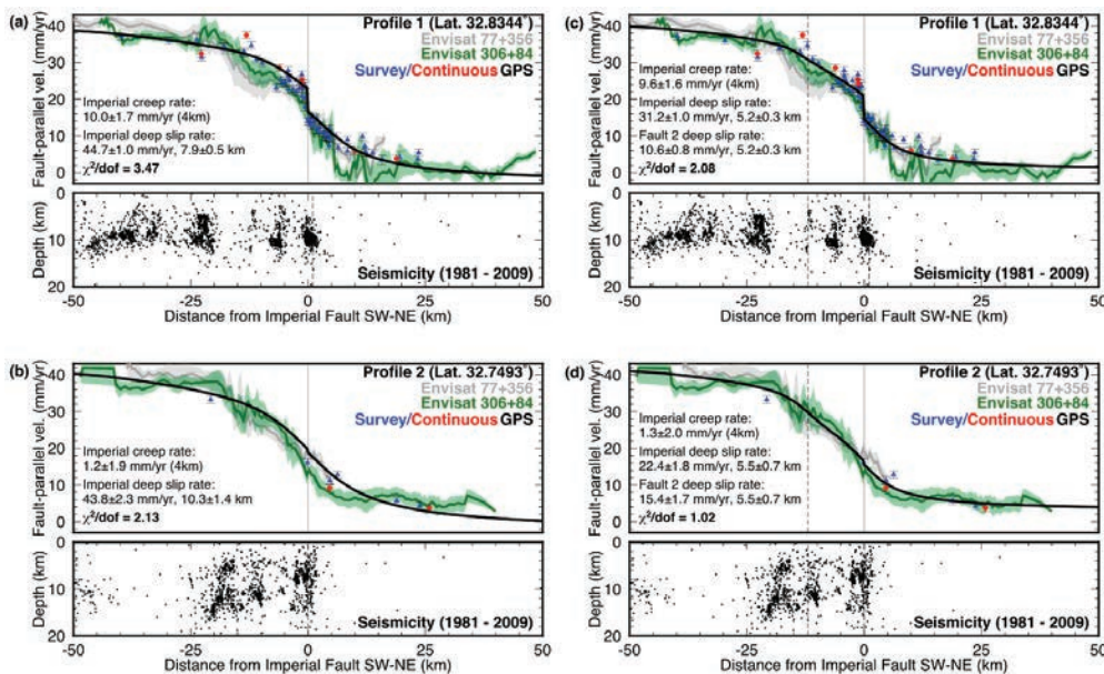
Figure 1: Proles across the Imperial Fault showing InSAR-derived fault-parallel velocities (gray and green curves), and GPS velocities from campaign (blue) and continuous stations (red). Black curves denote best-fitting models assuming one fault (a, b), and two faults (c, d). Fault locations are denoted by dashed lines. Model uncertainties are 2\sigma condence intervals. From Lindsey and Fialko [2016].
