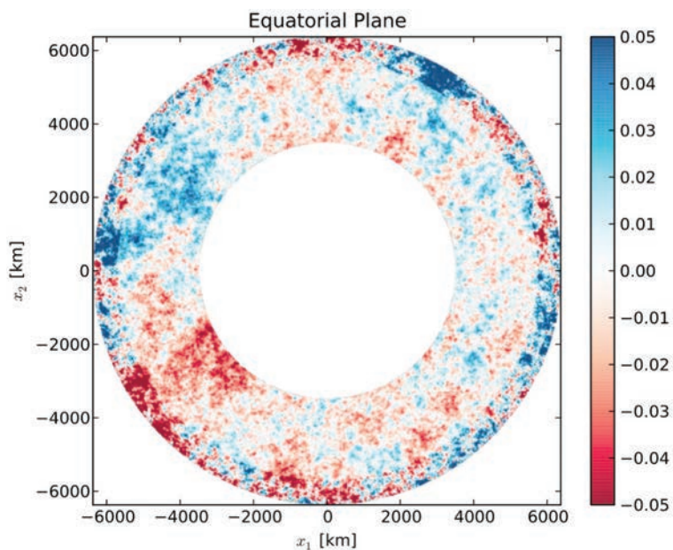
Figure 2. Cross section through an example 3-D mantle model with random heterogeneity. The 600-km-thick upper mantle has stronger heterogeneity than the lower mantle. The heterogeneity in both layers is a random realization of a Von Kármán autocorrelation function. The model shown here has much stronger lower mantle heterogeneity than we found is required to explain our P coda observations. Figure from Mancinelli et al. (2016).
