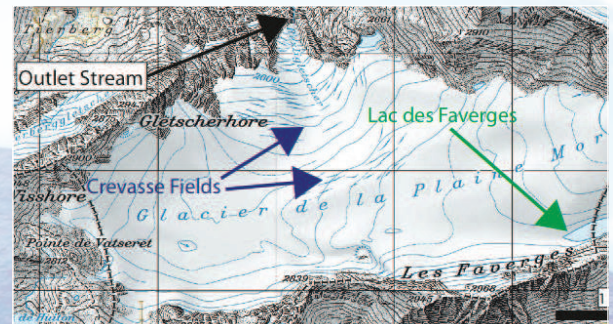
Figure 1: Map of Glacier de la Plaine Morte just south of Wildstrubel, Switzerland. The Rhone valley is to the south. Marked is the outlet stream at the toe of Rextliglacier that drains into the Simme river to the north. Arrows mark Lac des Faverges, a major glacier lake, and the two crevasse fields that Laske and Walter occupied with four arrays of short-period seismometers during the 2016 summer. The instruments were borrowed from the GIPP instrument pool at GFZ, Potsdam, Germany.
