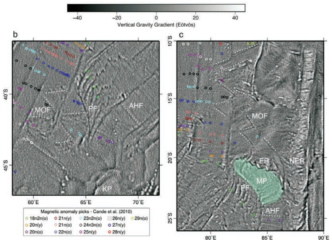
Figure 1. Vertical gradient of the marine gravity field reveals the detailed tectonics in the Indian Ocean ( Sandwell et al. , 2014; Matthews et al. , 2016). These gravity data were used along with plate reconstructions to discover the Mammerrickx Microplate which is the size of West Virginia (green shading on right figure).
