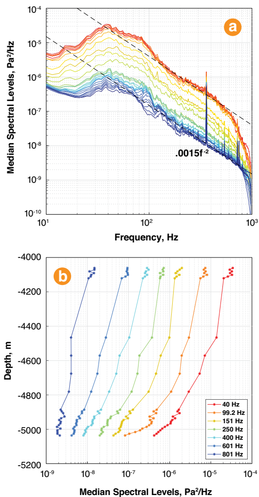
Figure 4. (a) The spectrum of the acoustic floor rises about 16 dB from the bottom element of the VLA (blue, 5036 m) to the top element (red, 4081m) for frequencies between 40 and 500 Hz. The lower dash line is the function 0.0015 \times f^{-2} ; the upper dash line is parallel and 16 dB higher. (b) The profile of the power up the array at selected frequencies shows the gradient is least at the highest frequency (blue) where the spectrum is smallest.
