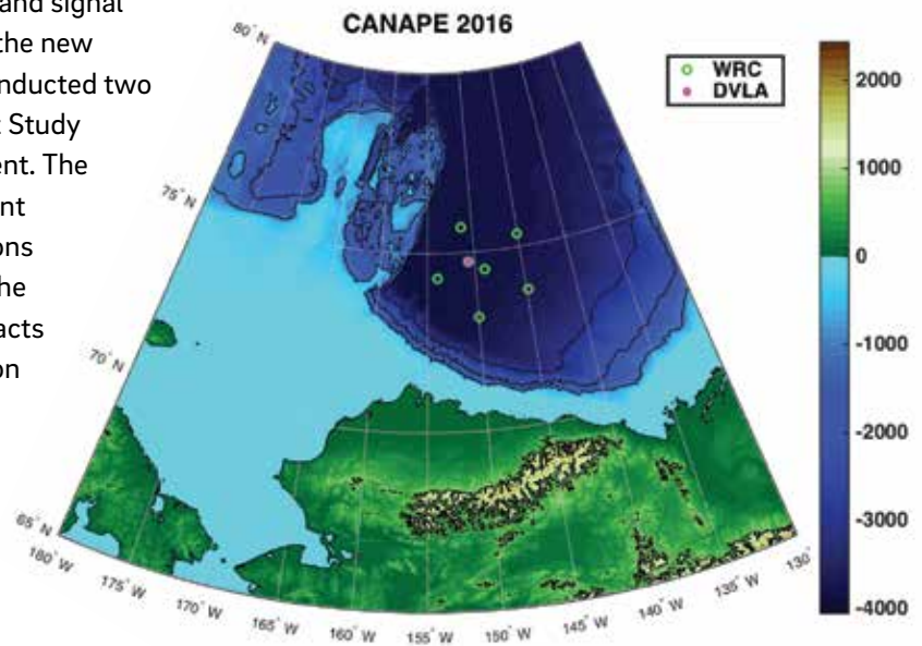
Figure 36. The 2016–2017 CANAPE experiment consisted of six Tele-dyne Webb Research acoustic transceivers (WRC, green) and a DVLA receiver (DVLA, red). The array radius is 150 km.
