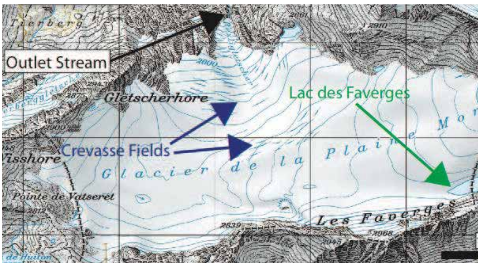
Figure 21. Map of Glacier de la Plaine Morte just south of Wildstrubel, Switzerland. The Rhone valley is to the south. Marked is the outlet stream at the toe of Rexpliglacier that drains into the Simme river to the north. Arrows mark Lac des Faverges, a major glacier lake, and the two crevasse fields that Laske and Walter occupied with four arrays of short-period seismometers during the 2016 summer. The instruments were borrowed from the GIPP instrument pool at GFZ, Potsdam, Germany.
