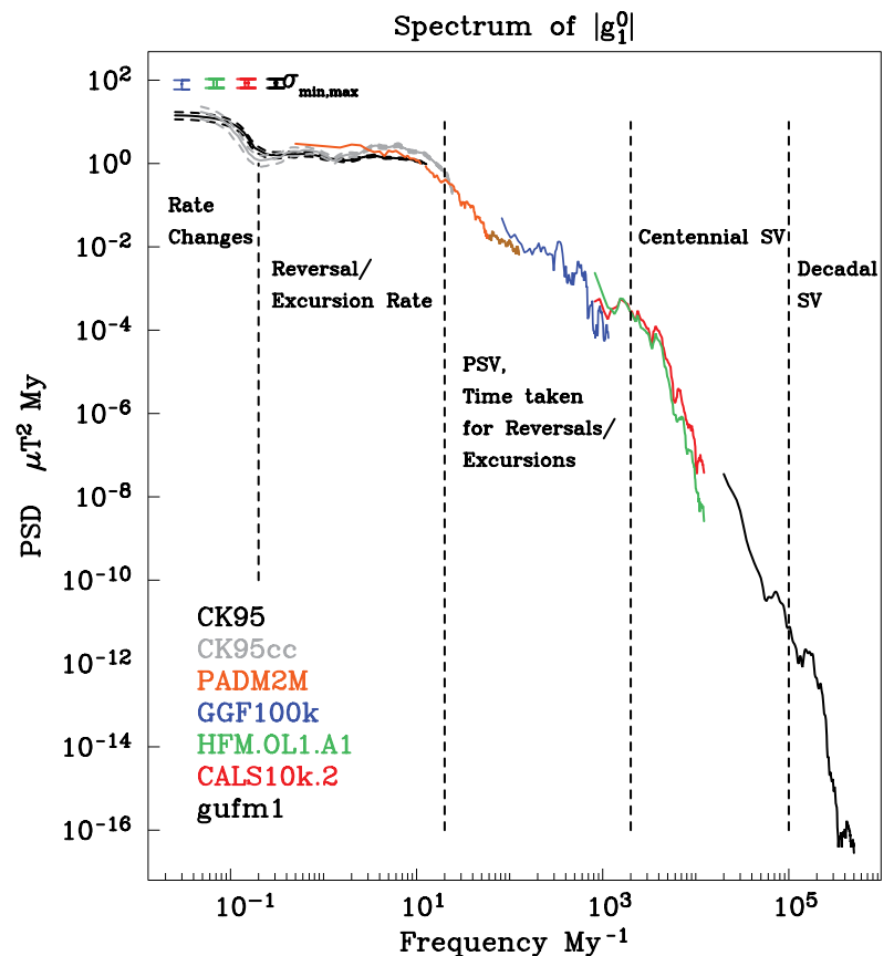
Figure 9. Power spectral density (PSD) estimates of the geomagnetic dipole moment from 0–160 Ma reversal record (CK95), 0–83 Ma reversal record including cryptochrons (CK95cc) 2 Ma paleomagnetic axial dipole moment reconstruction PADM2M, Holocene geomagnetic field models HFM.OL1.A1 and CALS10k.2, historical field model gufm1, and the new geomagnetic field model over the past 100 ka—GGF100k.
