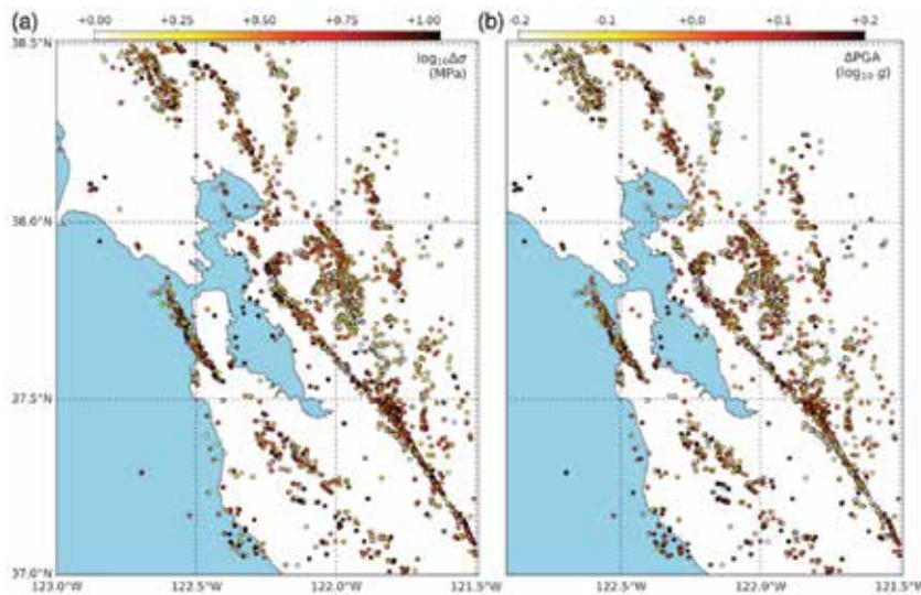
Figure 30. A comparison of spatial variations in: (a) estimated earthquake stress drops ( \Delta\sigma ), and (b) peak-ground-acceleration (PGA) residuals, for the San Francisco Bay region. Note the strong correlation between higher-than-average stress drops and higher-than-average PGA values, both plotted in red.
