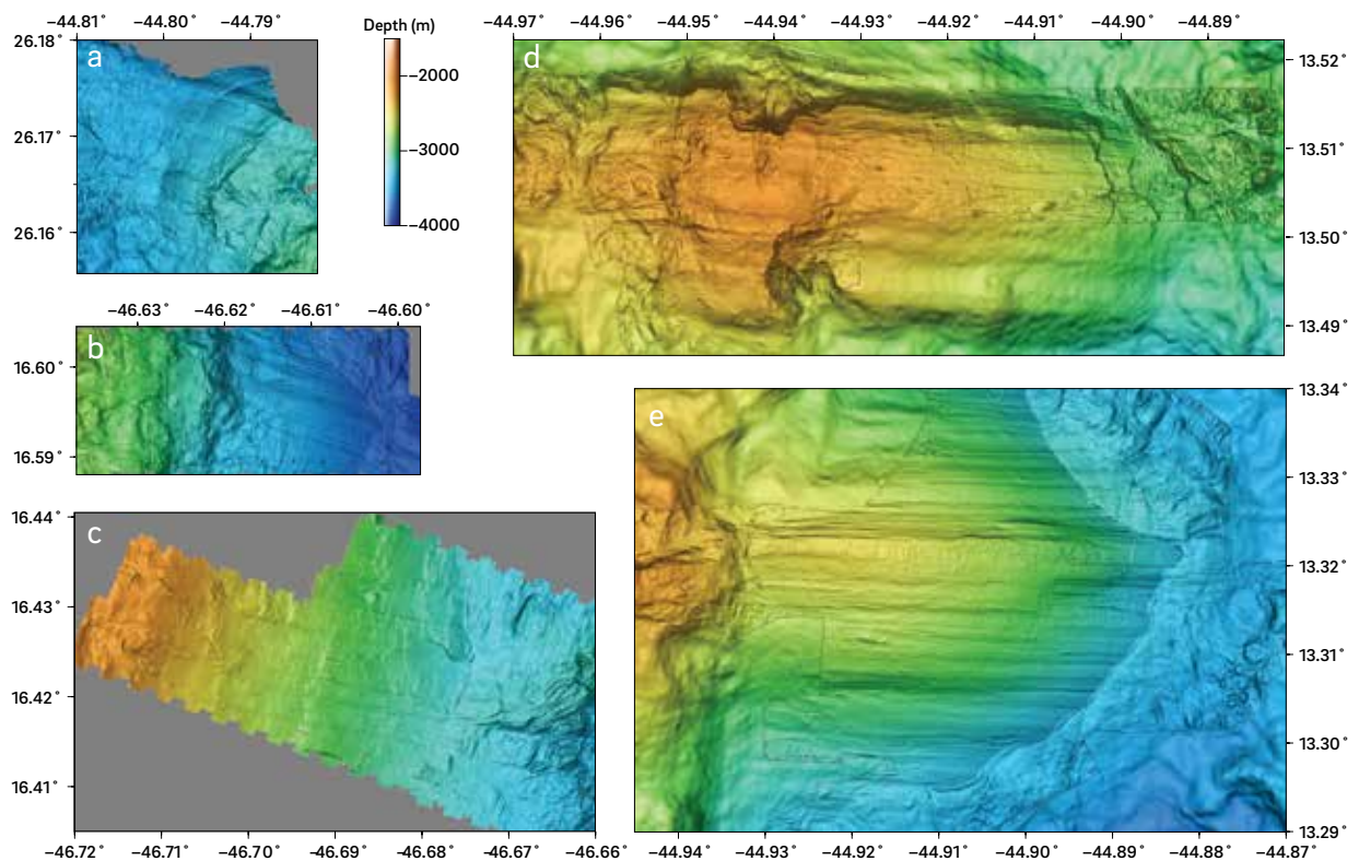
Figure 26. Bathymetric data collected at -60 m above seafloor over corrugated detachment fault surfaces, using AUVs on the Mid-Atlantic Ridge. a) Trans-Atlantic Geotraverse. b) and c) Near 16°N. d) and e) Near 13°30'N and 13°20'N. Arrows show inferred slip direction. Modified from Parnell-Turner et al. (2018a).
