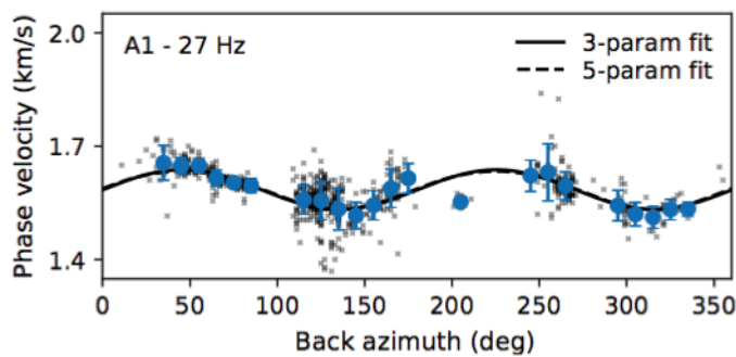
Figure 22. Measured azimuthal anisotropy at 27 Hz at array A1. Azimuthal anisotropy is modeled by a truncated trigonometric polynomial of degrees 2 and 4 in back azimuth. A decline of azimuthal anisotropy with decreasing frequency (not shown) indicates a shallow (20–30 m) origin for the anisotropy.
