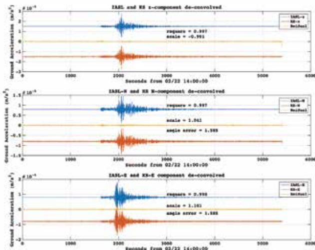
Figure 3. An example of a seismogram showing comparison between the optical seismometer, processed to convert mass position to ground acceleration, and the records from a co-located KS54000.
