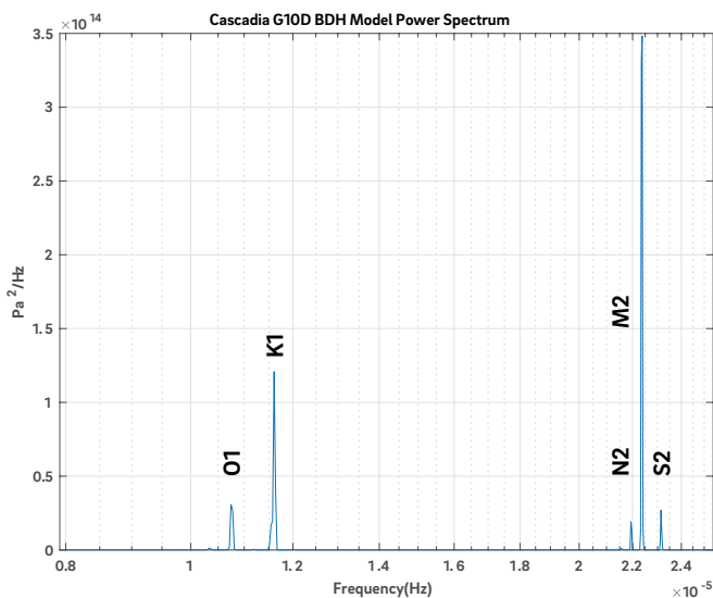
Figure 23. The power spectrum for the best fit tidal model obtained by using the Welch method is plotted in this figure.
