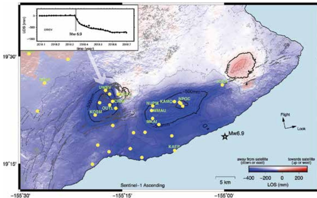
Figure 29. Line of sight (LOS) deformation associated with the 2018 Kilauea Hawaii event derived from Sentinel-1 InSAR and continuous cGPS (yellow dots). The event began on in late April as an eruption at the PuuOo crater which was followed by opening and dike injection on the East Rift Zone. This triggered a major earthquake (May 4, 2018, Mw6.9) on a shallowing dipping thrust fault ( https://www.usgs.gov/news/k-lauea-volcano-erupts ). Lava flows began along the lower East Rift zone and continued until late August 2018 destroying nearly 700 homes and displacing thousands of residents. We are working with colleagues at the University of Hawaii at Manoa to develop a complete deformation time series of this ongoing event ( http://pgf.soest.hawaii.edu/Kilauea_insar/ ).
