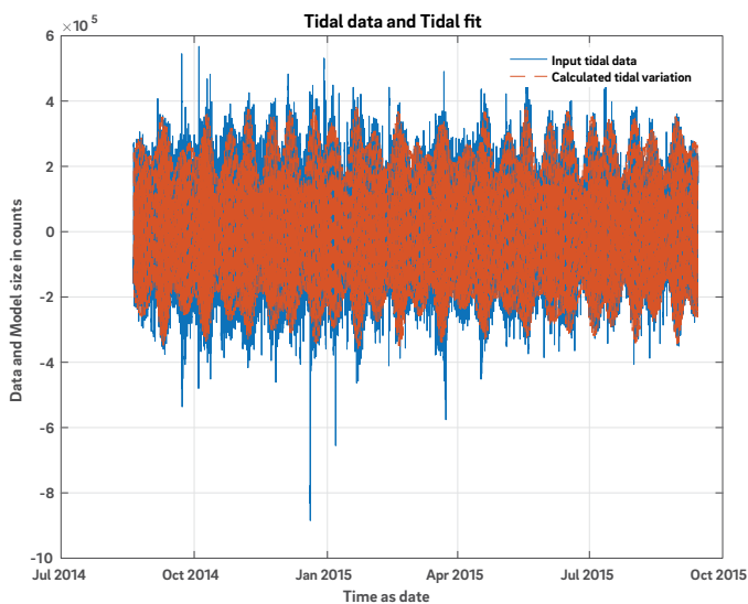
Figure 24. This figure overlays the best fitting tidal model (red) with the raw data (blue).
