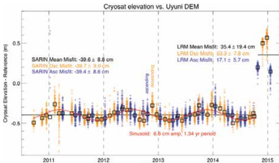
Figure 8. Left: Cryosat elevation validation relative to the salar de Uyuni DEM, with residuals showing a.) a uniform range bias of -40 cm for SARIN mode and +35 cm for LRM mode, b.) an 7 cm amplitude sinusoidal anomaly of 1.34 yr period that is still unexplained, and c.) higher range resolution than reported elsewhere, even with the sinusoidal anomaly. Right: ALOS InSAR results over the salar de Uyuni for the period 8/27/2010 - 1/12/2011, indicating that seasonal elevation change is <1 cm averaged over the salar surface.
