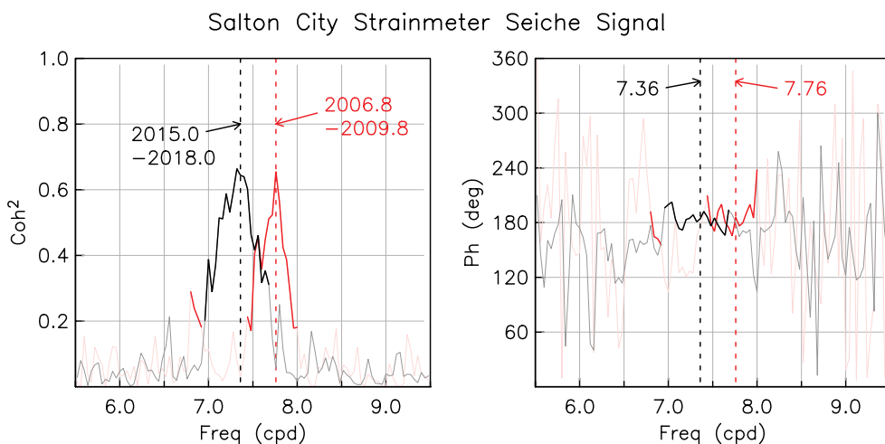
Figure 1. Coherence and phase between the NS and EW strain measurements at Salton City, for the first and last three years of the deployment. The peak in coherence is caused by loading from the gravest mode of oscillation in the Salton Sea.
