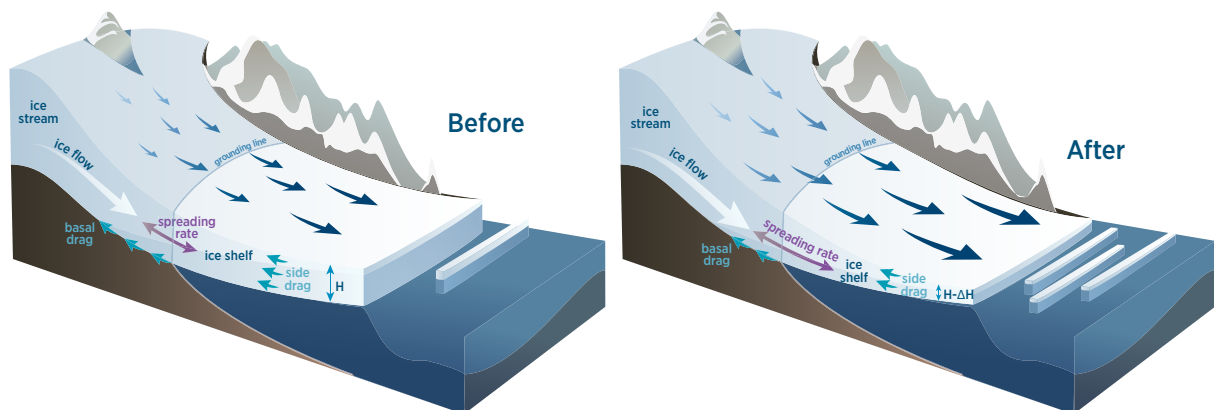
Figure 18. Ice shelf buttressing and GL flux. Confined ice shelves restrain the flow of upstream tributaries. Ice-shelf thinning increases the longitudinal stress and with it the spreading rate at the GL. This effect is felt some distance upstream, and net result is an increase in GL ice-flux.
