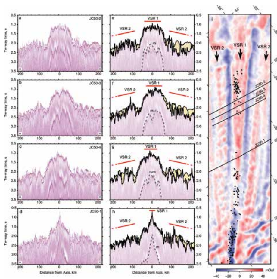
Figure 27. Portions of seismic reflection profiles crossing Reykjanes Ridge. (a–d) Profiles JC50-2, JC50-3, JC50-4, and JC50-1, respectively. (e–h) Interpretation: yellow shading = sedimentary cover, solid black lines = seabed and sediment-basement interface; labeled red lines = VSRs, m = seabed multiple. (i) Satellite free-air gravity anomaly map high-pass filtered to remove wavelengths >250 km. Labeled black lines = seismic profiles, black dots = relocated earthquakes between 1960 and 2009 ( M_w > 4 ); labeled arrows = VSRs. From Parnell-Turner et al. (2017a).
