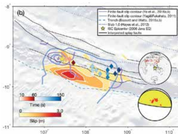
Figure 31. Seismic and tsunami back-propagation results and slip models of the 2006 Java earthquake (from Fan et al., 2017). Contours show two different finite-slip models. Diamonds show the peak-energy locations of high-frequency back-projection. Stations used for back-projection and their P-wave polarity with the GCMT focal-mechanism are shown as inserts. The subduction geometry is from Slab 1.0 with 20 km separation.
