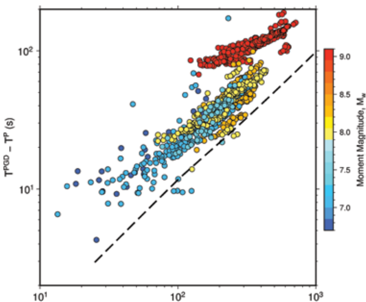
Figure 5. Relationship between hypocentral distance and the time from P-wave arrival to final peak ground displacement (TPGD-TP) for a series of Mw6.7 to Mw9.1 earthquakes in Japan from 2003 to 2016. Peak ground displacement is the first reliable metric for estimation of earthquake magnitude, thus this is indicative of how quickly accurate magnitude estimation is possible for large earthquakes. Black dashed line is the expected S-wave arrival minus P-wave arrival (S-P) time for a 1D velocity model and 25 km source depth. Each colored circle represents an observation from a single GNSS station, and is colored based on the magnitude of the observed earthquake (Goldberg et al., 2018).
