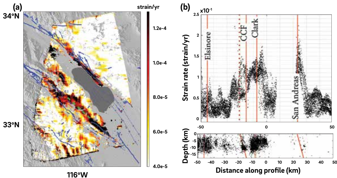
Figure 17. a) Maximum shear strain rates, obtained from regularized differentiation of the horizontal velocity data. The green rectangle outlines the profile across the faults, and the selected data points from the profile are shown in the next panels. b) Top panel shows the strain rate data selected from within the same area as the profile in panel a). The vertical red lines show the locations of each of the modeled faults at depth. The bottom panel shows the cross-section with seismicity denoted by black dots. From Tymofyeyeva and Fialko (2018).
