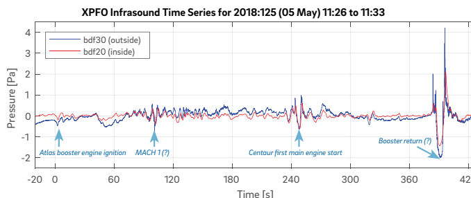
Figure 14. Infrasound sensors located at Pinyon Flat Observatory recorded the successful launch of the Mars INSIGHT mission from Vandenberg AFB on May 5, 2018. The pair of sensors, one with a flexible rosette hose filter (shown in red) and one with a rock pile noise reduction filter (shown in blue), recorded the event with differing quality. Courtesy C. Ebeling, Iceland). Photo courtesy C. Sites.
