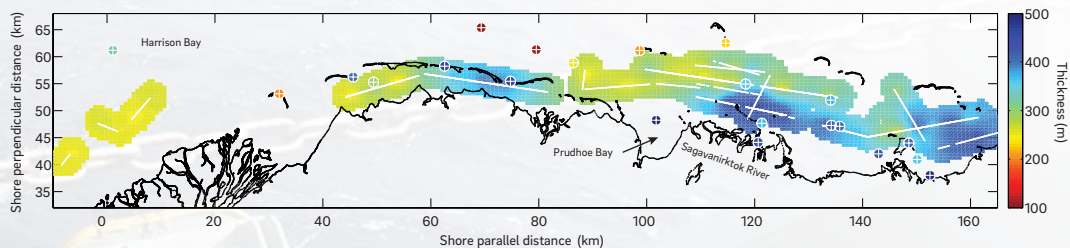
Figure 11. Map of permafrost thickness, offshore Prudhoe Bay, Alaska, measured using a novel surface-towed marine EM system developed by the marine EM lab.
