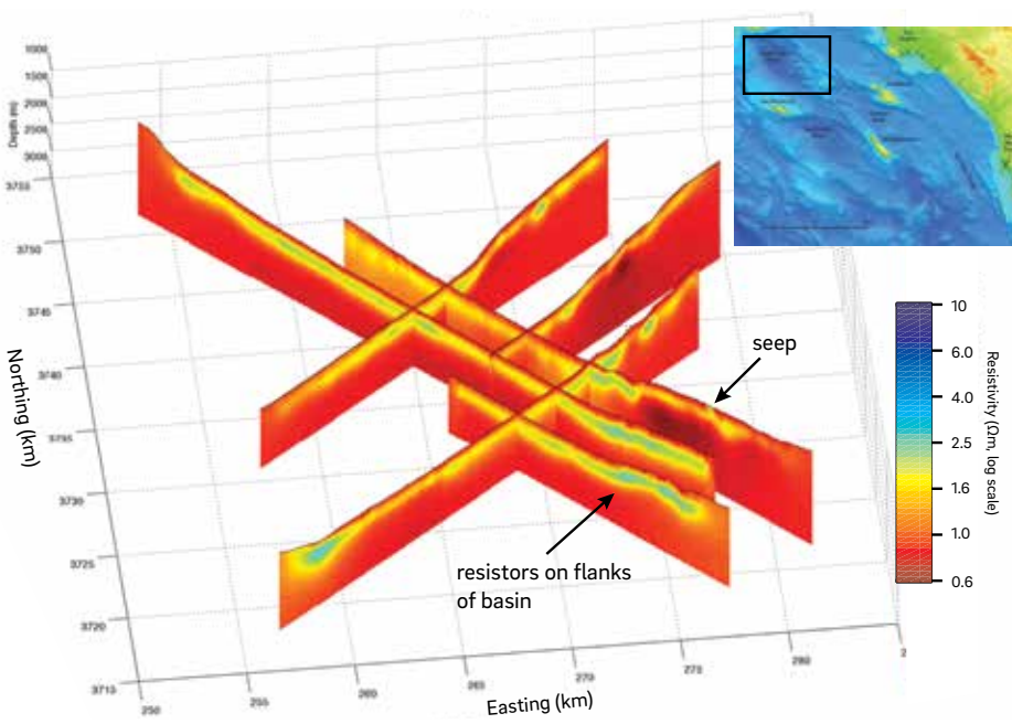
Figure 12. Electrical resistivity of the Santa Cruz Basin. Cool colors are resistors, showing that gas hydrate is associated with the flanks of the basin.
