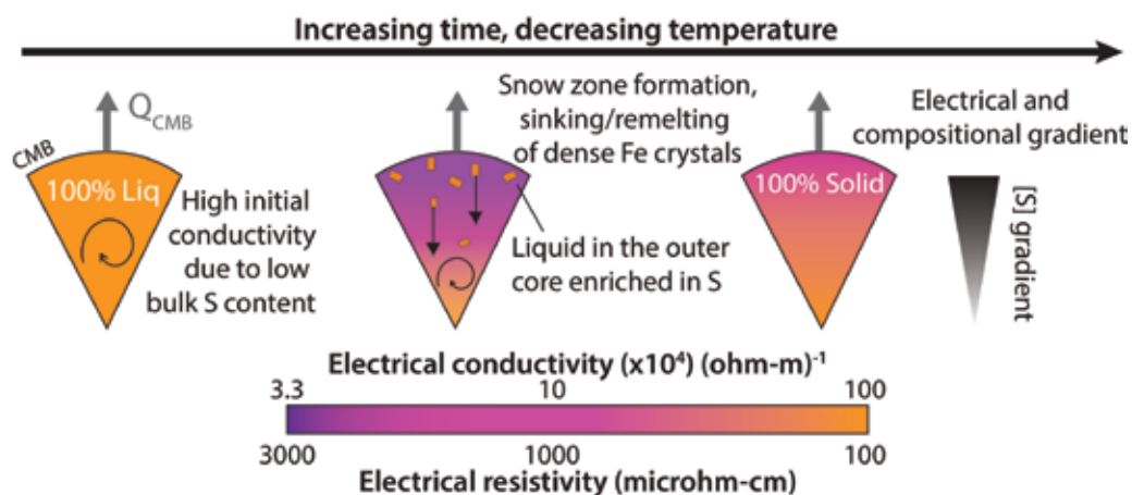
Figure 28. Example of top-down core crystallization and the evolution of the electrical response as chemistry and temperature change. Electrical resistivity values come from electrical experiments. In this example, pressure ranges from about 5 to 8 GPa, which is relevant to Ganymede's core (Pommier, 2018).
