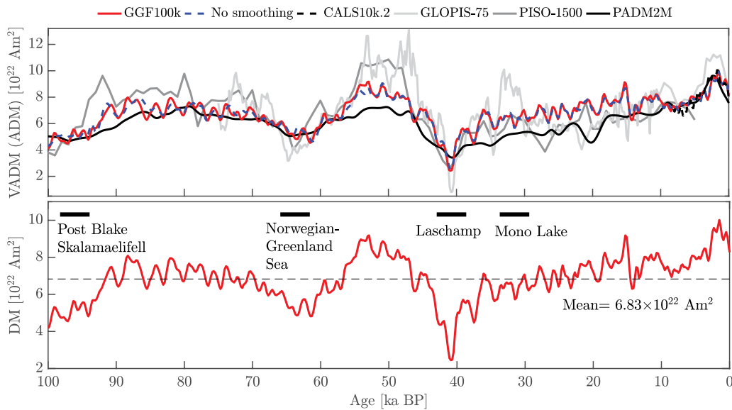
Figure 10. Dipole moment variations from 0-100 ka for GGF100k compared with earlier field models.
