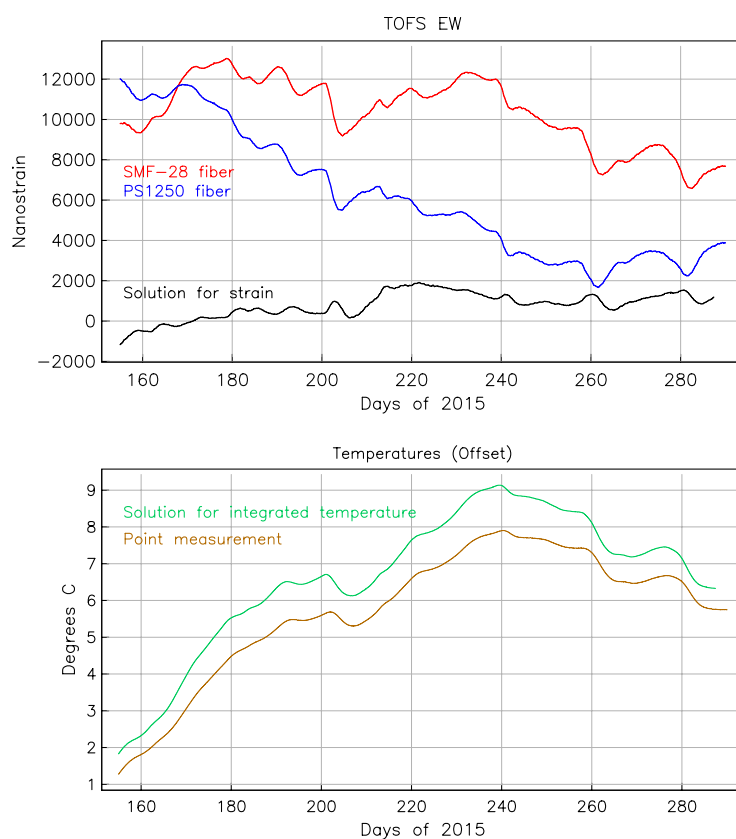
Figure 1. Data from the EW TOFS (Trench Optical-Fiber Strainmeter) installed at PFO. The upper panel shows the apparent strains observed on the two fibers, and the estimated strain from the temperature-neutral combination (black). The lower panel shows the estimated temperature and that measured at one point.
