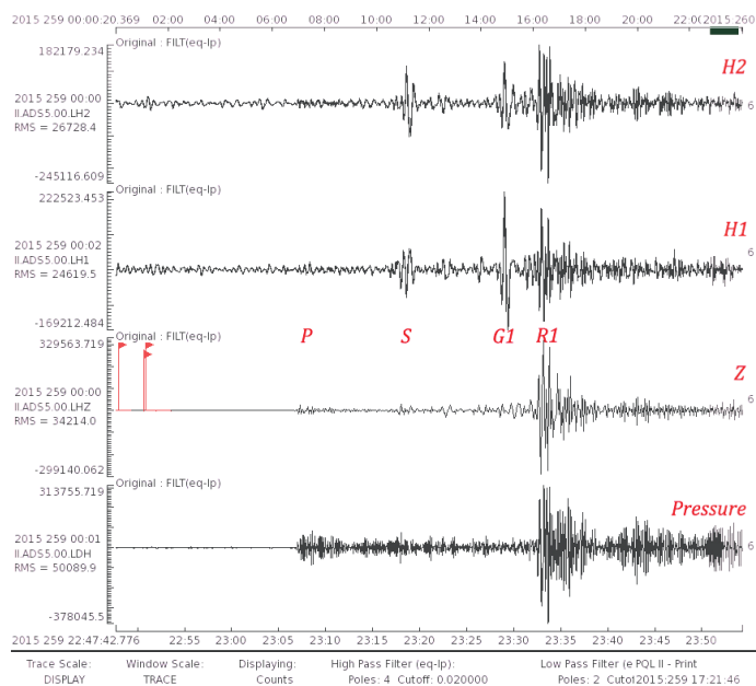
Figure 1. Near-real-time fourcomponent OBS time series of the of the great tsunamigenic Sep 16, 2015 Illapel, Chile earthquake. Top three traces are the two horizontal and the vertical component of a Nanometrics Trillium T-240 seismometer. The bottom record is from a differential pressure gauge (DPG) developed at SIO. The traces are bandpass filtered to emphasize long-period seismic waves. Laske and Programmer Analyst David Chavez witnessed how the waveform arrived on IGPP computer screens in near-real time.
