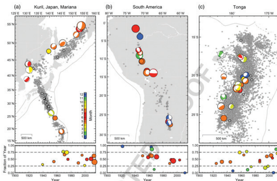
Figure 2. Regional plots of deep-focus earthquakes for the (a) NW Pacific, (b) South American, and (c) Tonga subduction zones. Events larger than M 7 are colored by month. Back-ground seismicity is shown as small grey dots. (bottom row) Event month versus year. Symbol sizes are proportional to magnitude.
